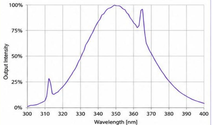
UV Spectrum
